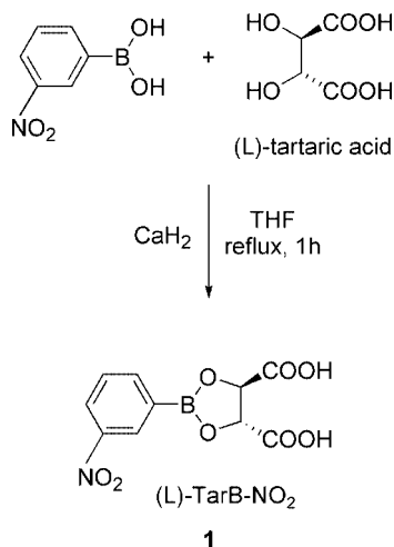
Scheme 1. Preparation of TarB-NO 2 reagent.
