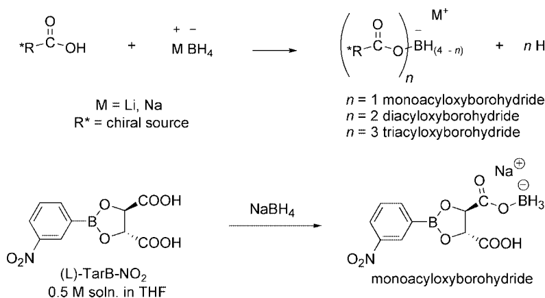
Scheme 2. Generation of a generic acyloxyborohydride and (L)-TarB-NO 2 monoacyloxyborohydride.
