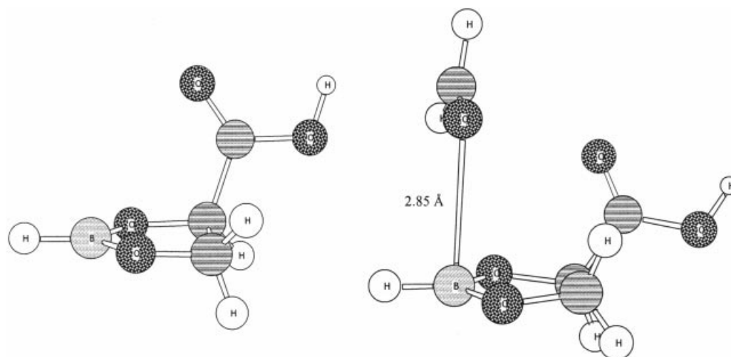
Figure 1. 1,3,2-Dioxaborolane-4-carboxylic acid and proximal formaldehyde complex (HF/6-31G*). Unlabelled atoms represent carbon.
