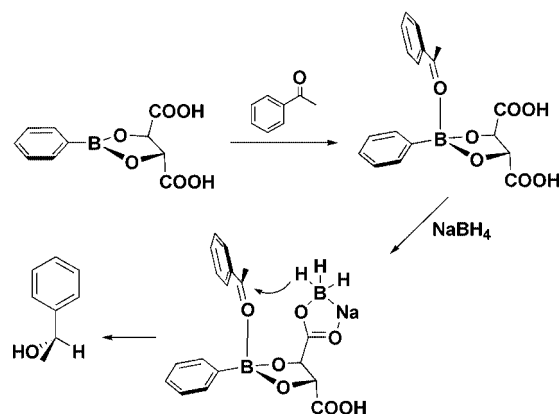
Scheme 3. Proposed mechanism for reduction of acetophenone by TarB-NO 2 .
