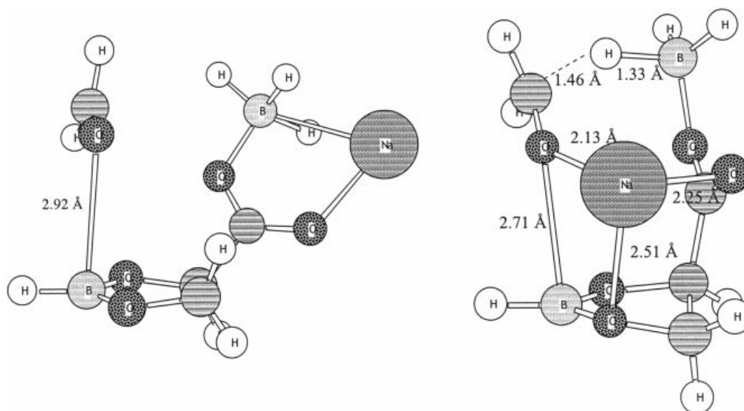
Figure 2. Sodium complex and the proximal transition state (HF/6-31G*). Unlabelled atoms represent carbon.
